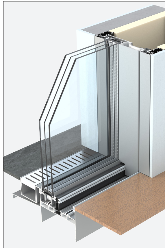
ARTLINE XL Pocket solution
