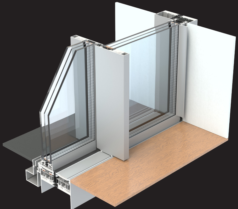
ARTLINE XL Flush: Super minimalistic sliding door with smallest sightline at the meeting stile
